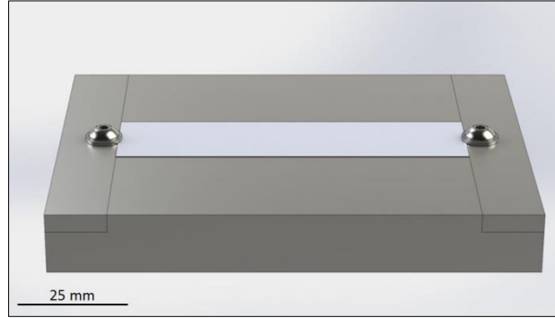
Figure 4-2 Almen strip fixture.
