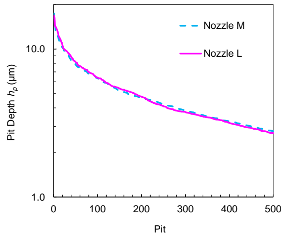
Figure 5-19 Pit depth as a function of nozzle dimension ( V_{in}=150 m/s, V_{out}=11.0 m/s and s_N=45 , t_E=5 s).
