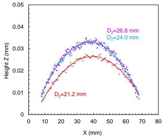
Figure 5-13 Net strip profiles for different outer flow diameters D_2 ( D_1 = 0.85 mm, V_{in} = 150 m/s, V_{out} = 11.0 m/s, Al 7075-T651, t_P = 18 min).
