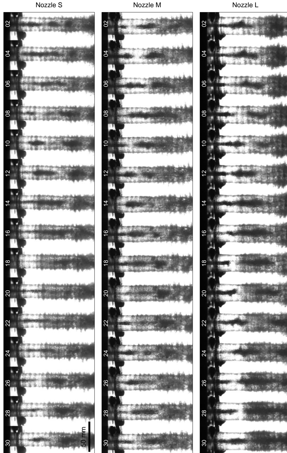
Figure 5-25 Sequence of 15 images of the cavitating flow for different nozzle sizes (constant D_1 ; D_0 ; D_2 ). This sequence represents every second image of videos captured at 14000 fps; the interval between frames is 143 \mu s ( V_{in} = 150 m/s, V_{out} = 11.0 m/s, frame numbers shown).
