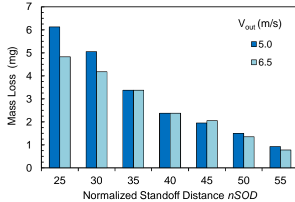
Figure 4-16 Mass loss in center regime as a function of outer flow velocity V_{out} and standoff distance s_n . ( V_{in} = 150 m/s, t_e = 3 min).
