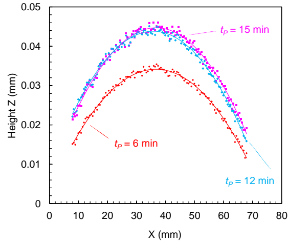
Figure 5-20 Net strip profiles for different processing times t_p (Nozzle L, V_{in}= 150 m/s, V_{out}= 11.0 m/s, s_N = 45 , Al7075-T651).
