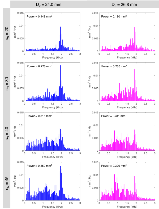
Figure 5-16 Power Spectral Density (PSD) of the cloud width variation as a function of time for different D_2 and different normalized standoff distances s_N .
